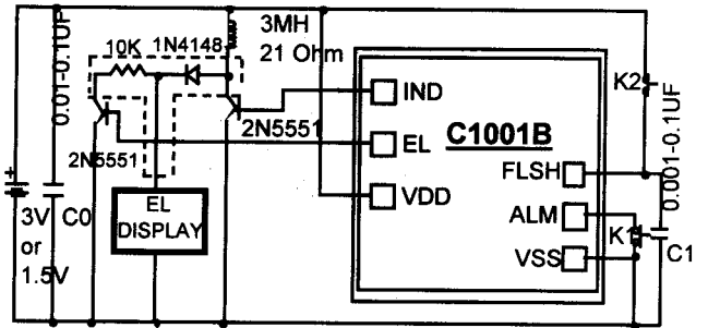
B. Application with 3 Second Delay using Vss Trigger & without Delay using FLSH Trigger
