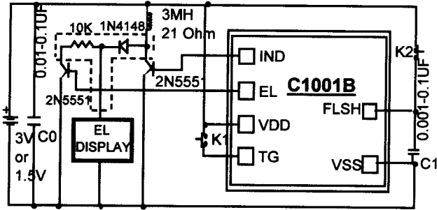
A. Application with 3 Second Delay using Vdd Trigger & without Delay using FLSH Trigger
