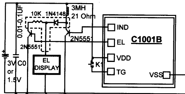
C. Application with 3 Second Delay using Vdd Trigger
