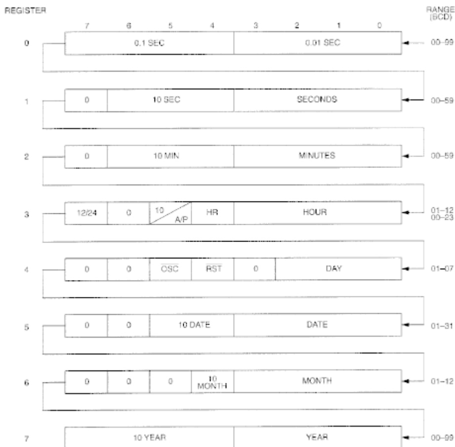
Figure 2. PHANTOM CLOCK REGISTER DEFINITION
