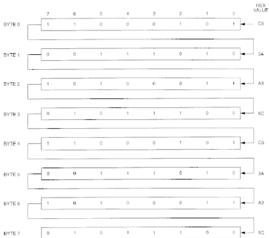
Figure 1. PHANTOM CLOCK REGISTER DEFINITION
